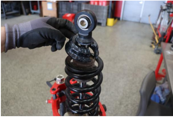
Step 7. Remove the spring retainer.
