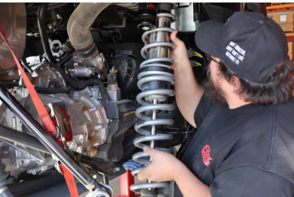
Step 17. Set shock assembly in vehicle by inserting top of assembly through opening in body panels and setting lower shock mount in trailing arm.
