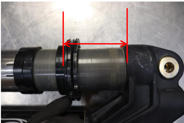
Step 11. Set pre-load of spring seat to 85mm (3 11/32in.) from bottom of seat to bottom of reservoir bridge.
