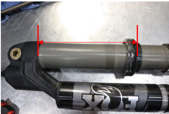
Step 11. Set pre-load to 190mm (7 1/2in.) from bottom of spring seat to bottom of furthest point on reservoir bridge. (Reservoir bridge is not flat relative to spring seat. Be sure to measure from the side opposite the reservoir).
